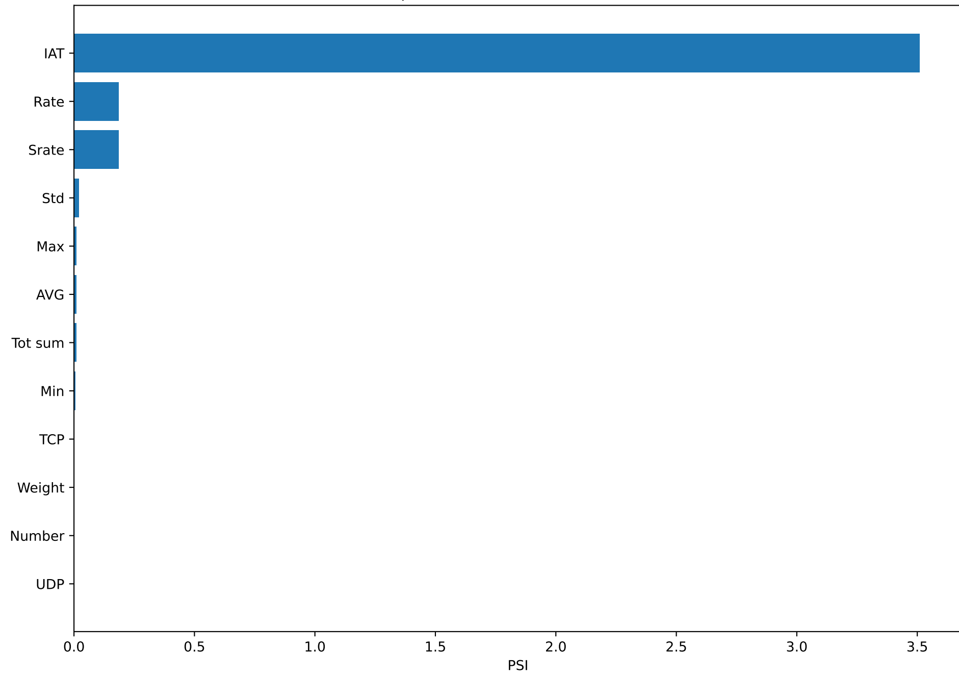
Top Train/Test Drift Features (PSI)
