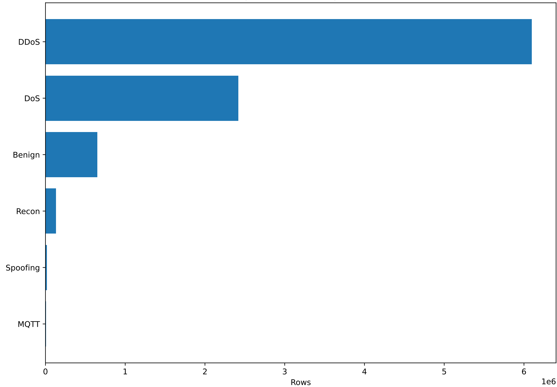
Top Attack Families by Rows
